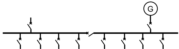
fig. 15: diagram of a network with local generation.
