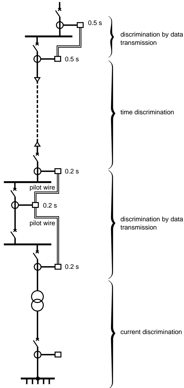
fig. 4: protection system using several discrimination techniques: current, time and logic.
