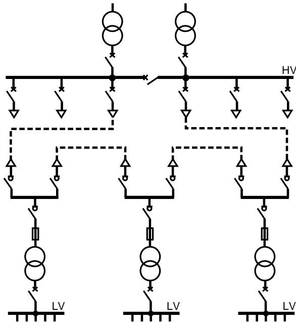
fig. 10: diagram of a primary loop.
