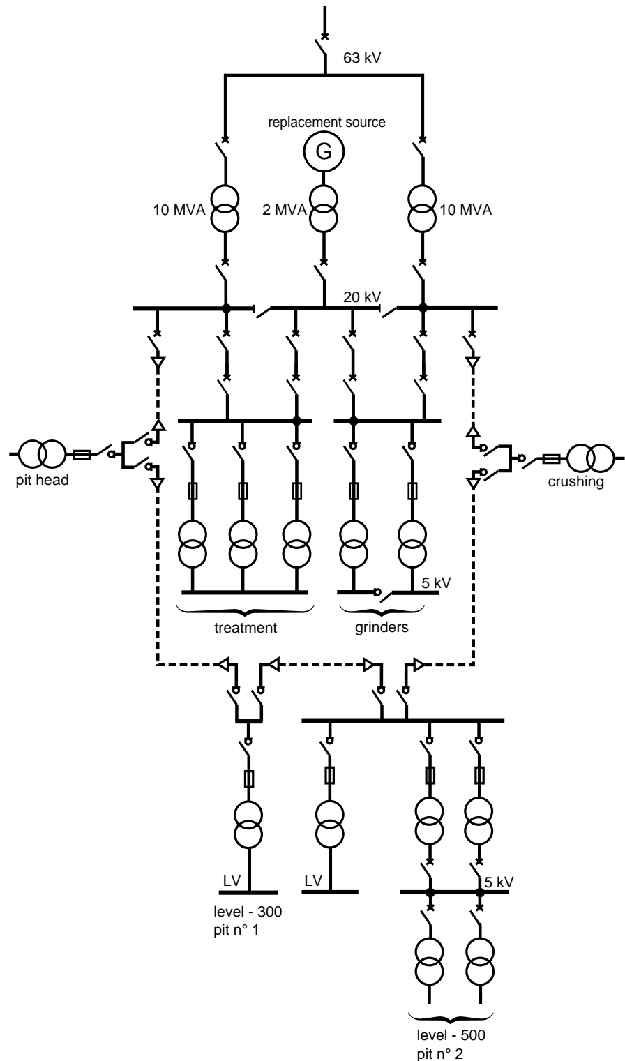
fig. 17: structure of the electrical network of a Moroccan mine (Merlin Gerin).
