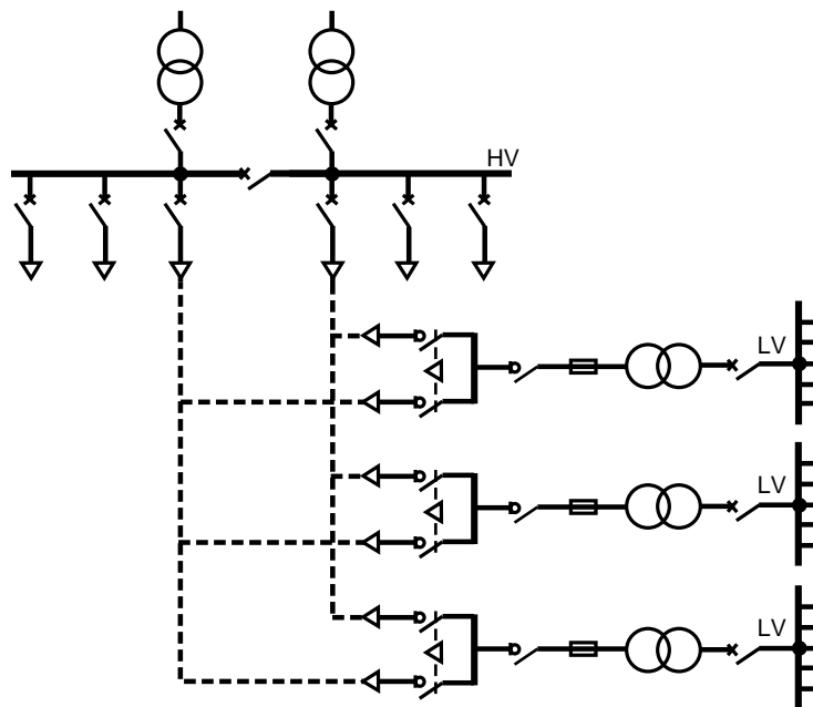
fig. 11: diagram of a primary selective network.
