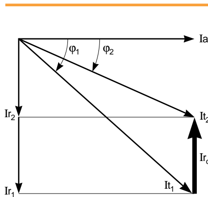
fig. 20: phasor diagram of the different currents and the effect of compensation.
