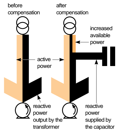
fig. 21: diagram depicting the energy exchange in a consumer circuit and the advantage of compensation.
