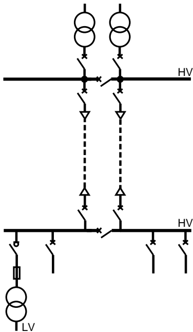
fig. 13: diagram of a dual power supply network.
