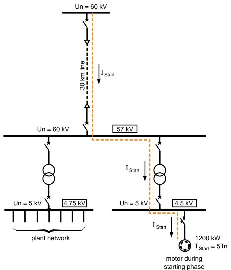
fig. 5: example of the determination of voltage dips during motor starting for the installation of a 1200 kW motor supplied by a 30 km long, 60 kV line. It should be noted that separation of the "plant network" power supply and the motor power supply have made it possible to have a voltage drop of only 250 V in the "plant network".
