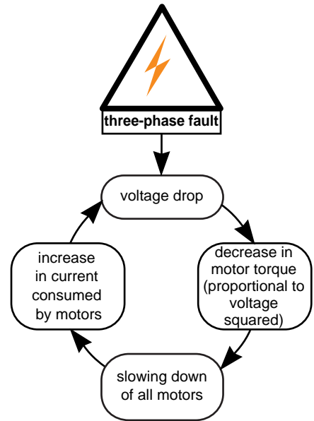
fig. 8: performance of asynchronous motors in the presence of a three-phase fault
