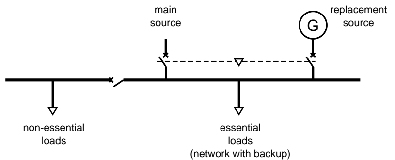
fig. 16: diagram of a network with a replacement source and load shedding.
