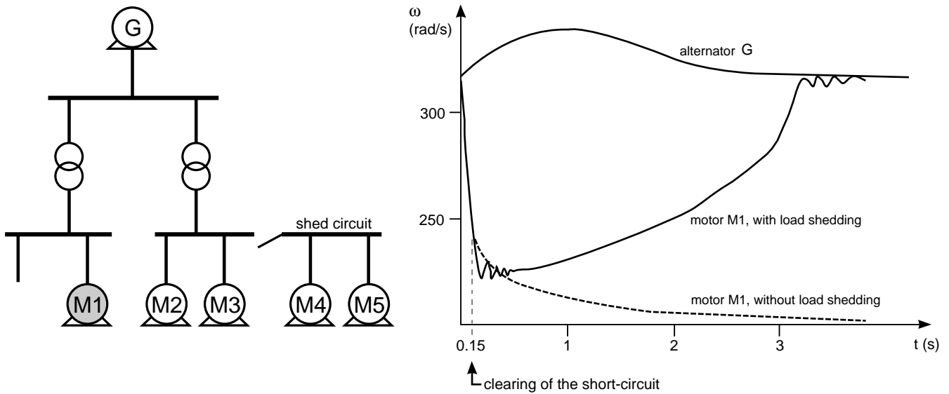
fig. 9: presentation of the dynamic performance of a network with and without load shedding
