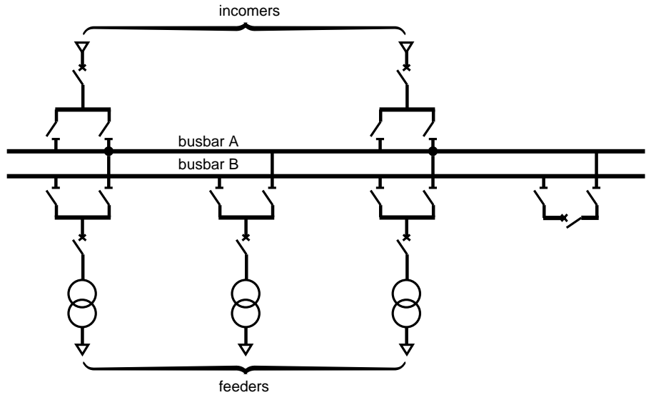
fig. 14: diagram of a dual busbar network.
