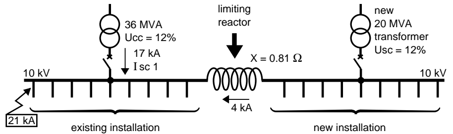
fig. 19: extension of an existing industrial network by addition of an extra transformer.
