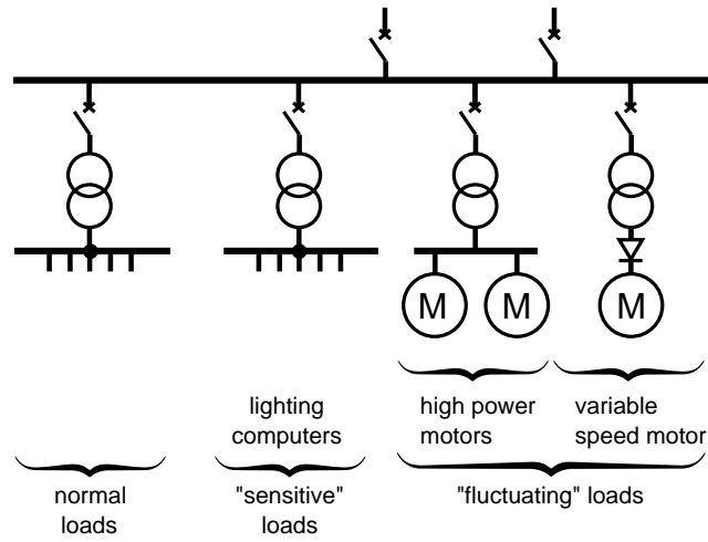
fig. 3: the division of sources is a means of separating the "fluctuating" loads from the other loads.
