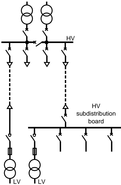
fig. 12: diagram of a single power supply network.
