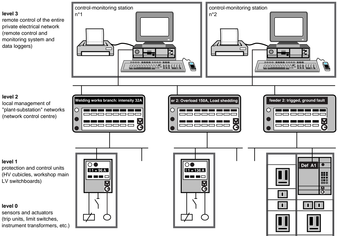
fig. 18: example of Energy Management System architecture.
