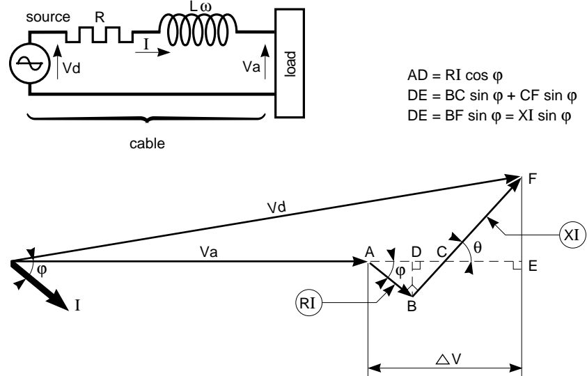
fig. 23: phasor diagram of network voltage drop
